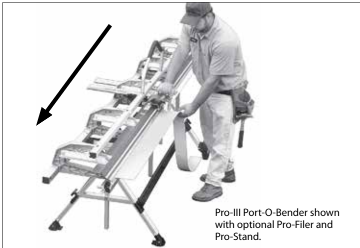
Figure 3. Use proper technique to push CUT-OFF through the material with a smooth, constant motion from right to left. Do not stop in the middle or cut with a back and forth motion. Use a piece or two of scrap material to practice.
