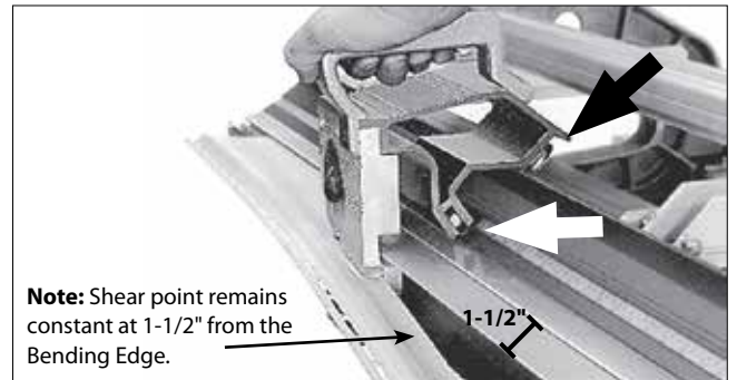
Figure 2. Engage Guide Rollers correctly. Make sure both front and back rollers are seated in their tracks. Note: large arrows in illustration above.
